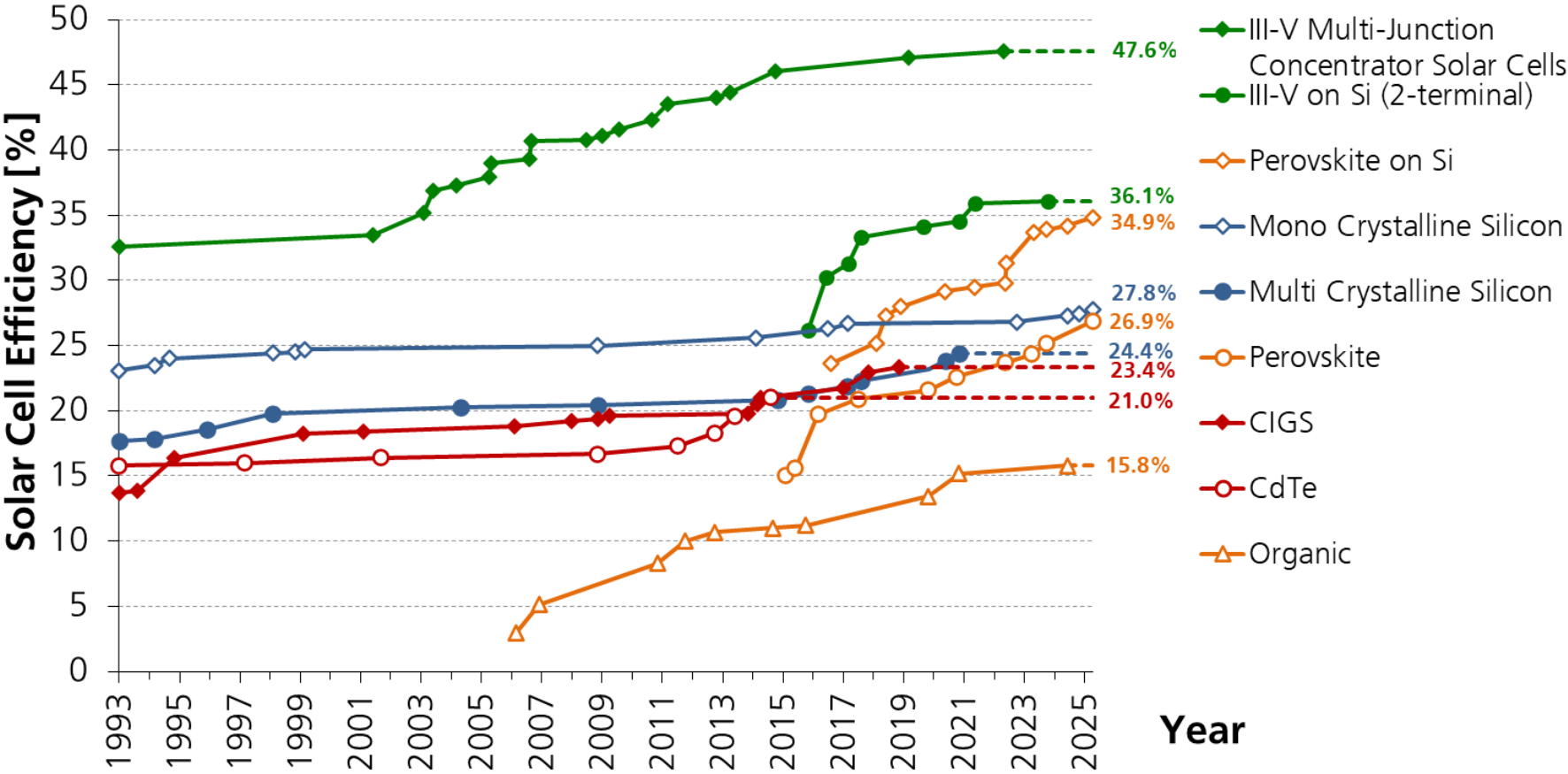
Data: Solar Cell Efficiency Tables (Versions 1 to 66), Progress in Photovoltaics: Research and Applications, 1993-2025. Graph: Fraunhofer ISE 2025. Date of data: 04/2025
